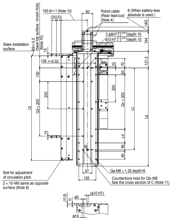
Cross section of C
